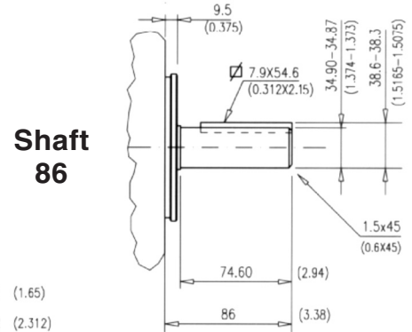
max torque capability: 600 Nm (5300 lb. in.)
