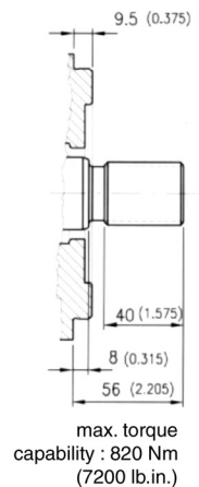
max. torque capability : 820 Nm (7200 lb.in.)
