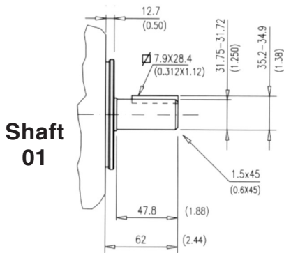
max. torque capability : 600 Nm (5300 lb.in.)
