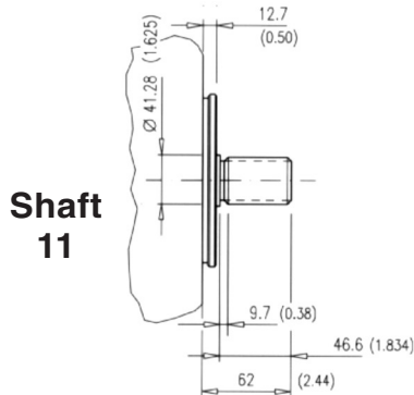
max. torque capability : 820 Nm (7200 lb.in.)
